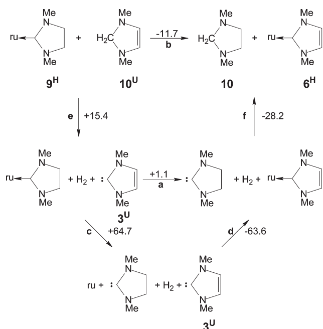
Scheme 2 Energies in kcal mol -1 ; ru = \text{RuHCl}(\text{PH}_3)_2
